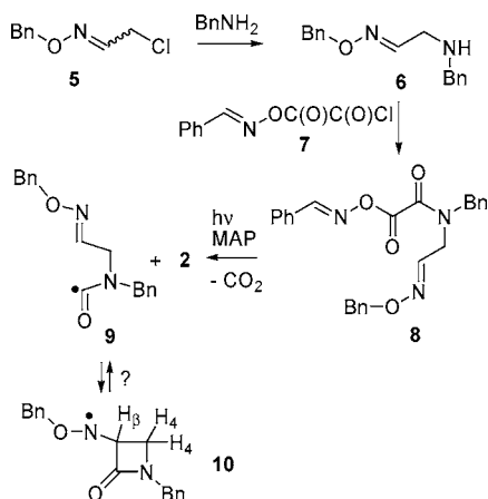
Scheme 2. Preparation of an Oxime Oxalate Amide with an Oxime Ether Side Chain and Formation of a Cyclized Oxyaminyl Radical
