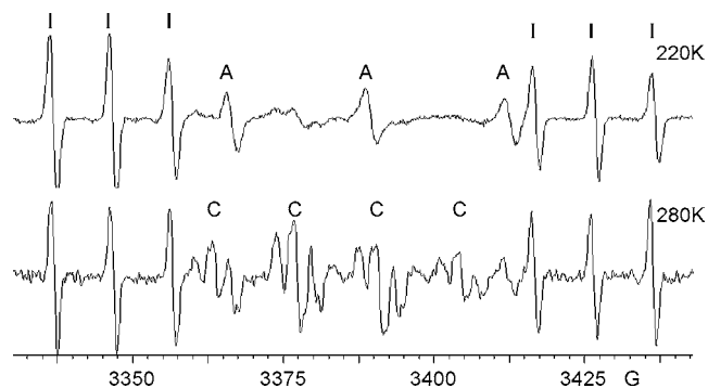
Figure 2. EPR spectra of radicals derived from 8 at 220 and 280 K in PhBu- t . I = iminyl 2 , A = carbamoyl 9 , C = aminyl 10 .
