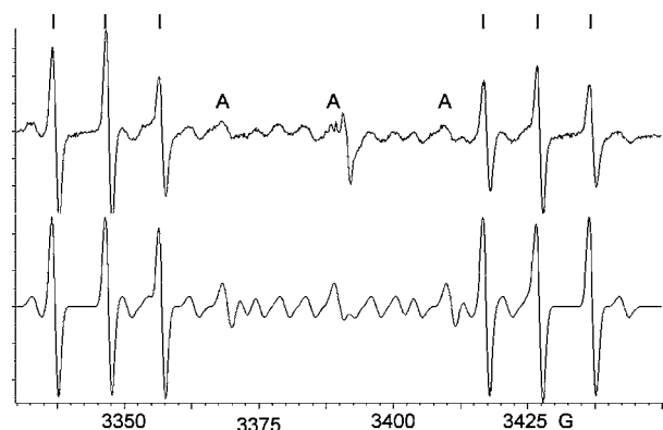
Figure 1. Top: EPR spectrum of radicals derived from 1 at 220 K in tert -butylbenzene. I = iminyl radical 2 ; A = aminoacyl (carbamoyl) radical 3 ; other lines are from cyclized radical 4 . Bottom: computer simulation.
